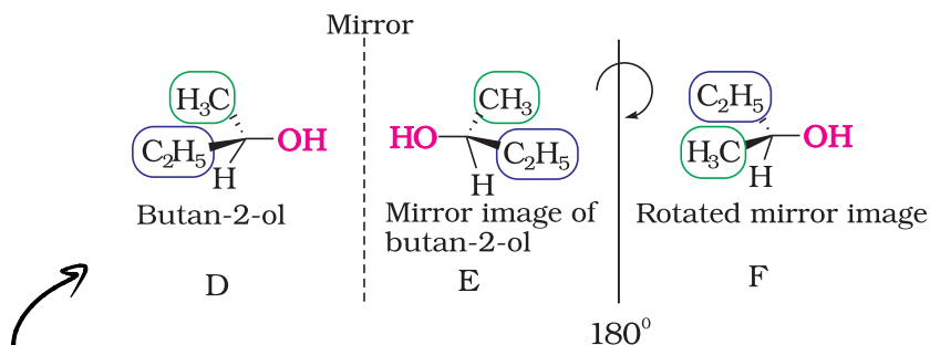
Fig 6.6: E is mirror image of D; E is rotated by 180^\circ to get F and F is non superimposable on its mirror image D.
